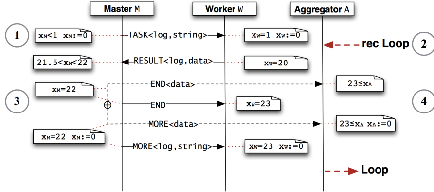
Fig. 1. Global protocol for log crawling in Scribble
