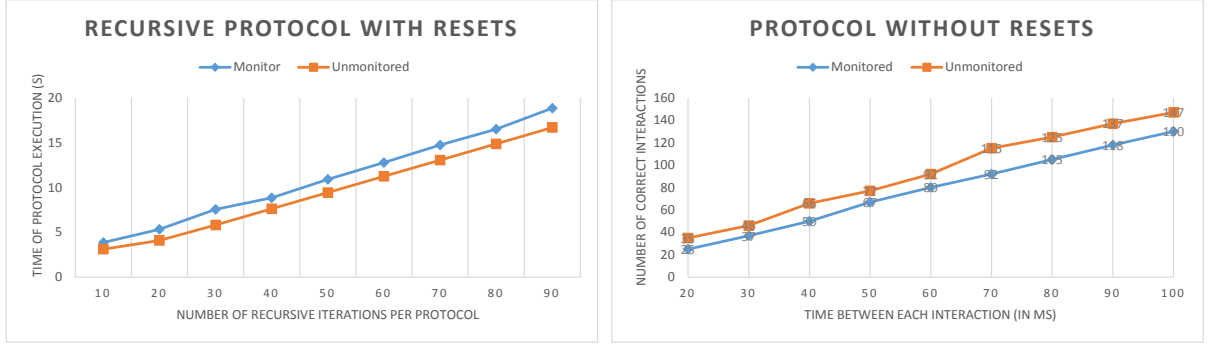
(a) The execution time per number of recursions for the protocol in Figure 15 (b) The maximum number of correct interactions for the protocol in Figure 17
