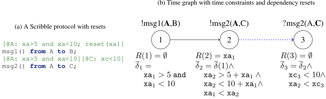
Fig. 12. An example of clock resets
