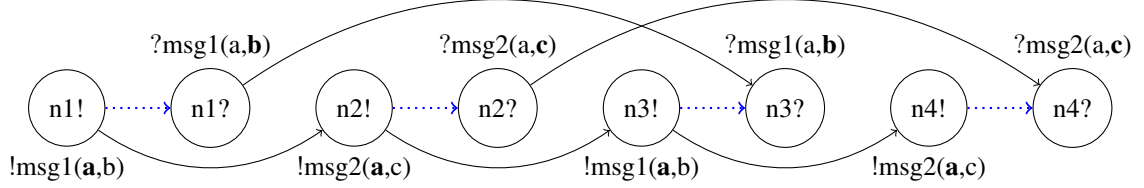
Fig. 10. Dependency graph for the protocol in Figure 9
