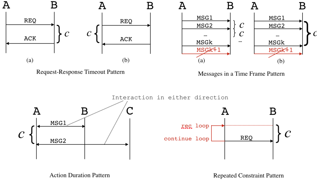
Fig. 18. An illustrated summary of the timed patterns
