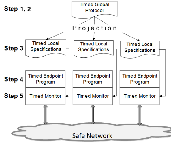
Fig. 2. Scribble toolchain framework
