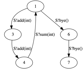
Fig. 5: A Screenshot of the \nu SCR Web Interface, Showing an Adder Protocol
